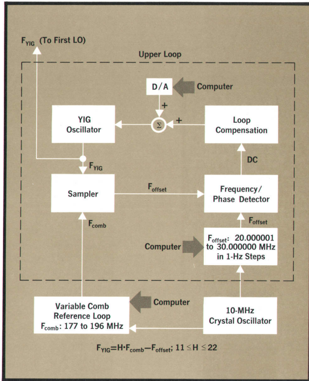
Fig. 3. Block diagram of the first local oscillator. F_{VIG} = H \cdot F_{comb} - F_{offset} ; 11 \leq H \leq 22 . F_{VIG} is coarse-tuned to harmonic H by the computer.
